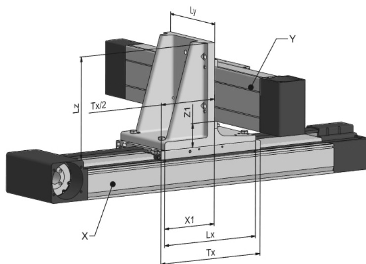
Figure 6.12 ____ Angle connections x – y – Axis system, profile assembly
