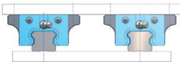
Two-rail arrangement (2)
