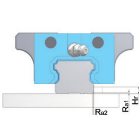
Figure 3.2. Locating edge of the carriages
