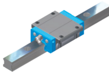
LGBCS...FN, standard
