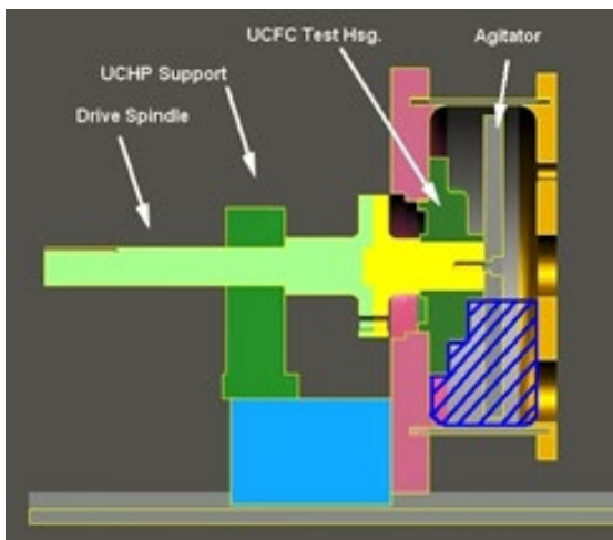
Contamination machine setup
